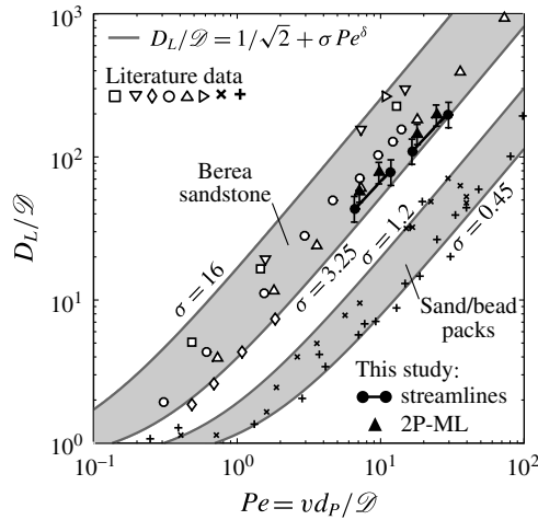
FIGURE 9. Dispersion data plotted as a reduced longitudinal dispersion coefficient ( D_L/D ) as a function of the Péclet number, Pe = vd_p/D , where D is the molecular diffusion coefficient, v is the interstitial (pore) fluid velocity and d_p is the average particle (or grain) diameter. The solid lines are obtained from a common correlation found in the literature (Sahimi et al. 1986), i.e. D_L/D = 1/\sqrt{2} + \sigma Pe^\delta , with \delta = 1.2 and \sigma = 0.45, 1.2, 3.25, 16 . Literature data are represented by the symbols and include measurements on sand/bead packs, i.e. (+) Dullien (1992) and (×) Perkins & Johnston (1963), as well as those on Berea sandstone samples, i.e. (□) Brigham et al. (1961), (▷) Scheidegger (1974) (after Cortis & Berkowitz (2005)), (▽) Baker (1977), (△) Hulin & Plona (1989), (○) Gist et al. (1990) and (◇) Honari et al. (2015). Results from this study are given by the black-filled symbols, as obtained from the ‘tuned streamtubes’ (●) and ‘2P-ML’ (▲) models and by assuming D = 1 \times 10^{-5} \text{ cm}^2 \text{ s}^{-1} and d_p = 150 \text{ }\mu\text{m} .
